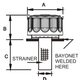
WELD TYPE
