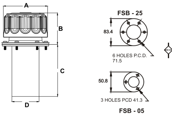
FLANGE TYPE
